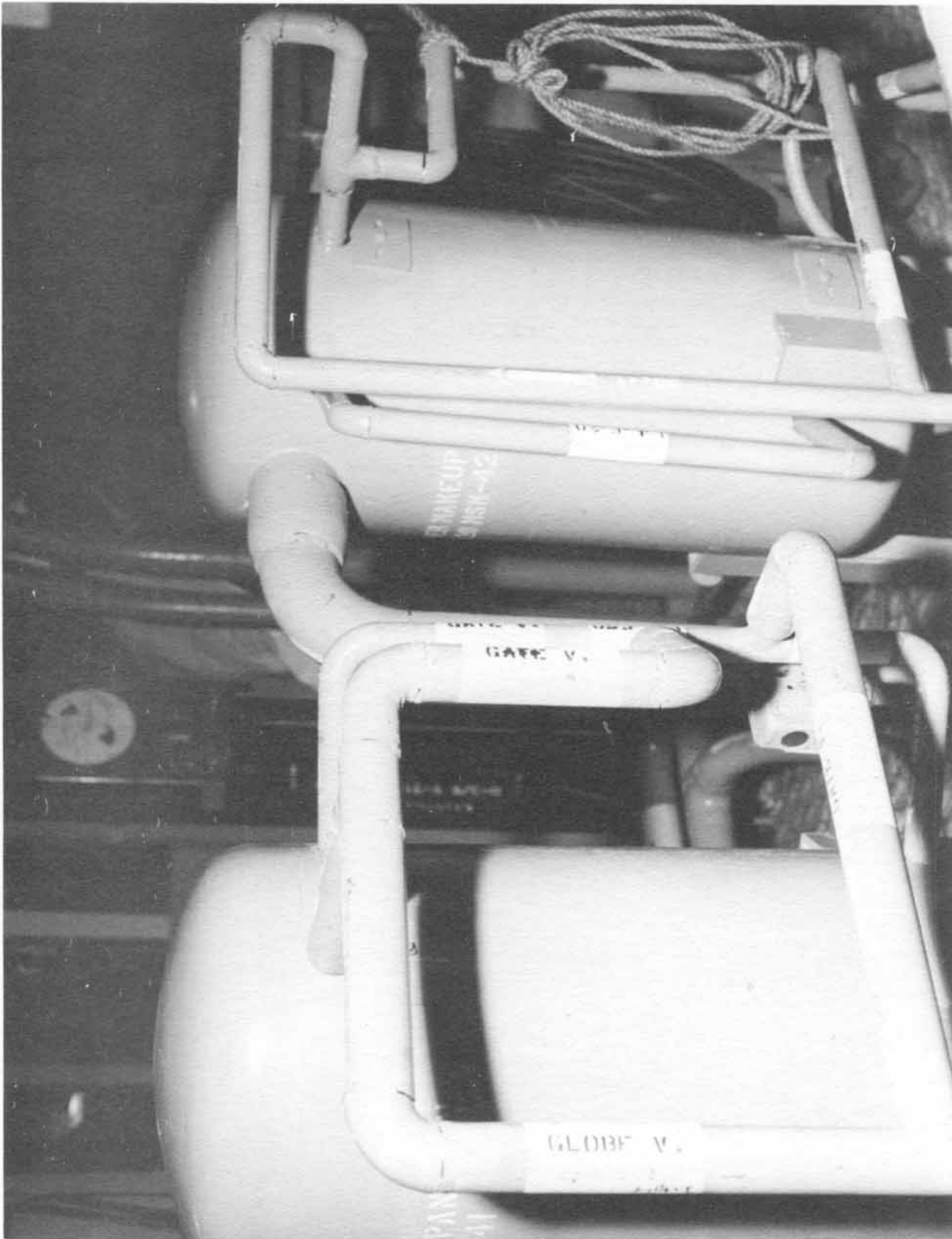
Chilled water and makeup tanks, Q-3, looking toward missile shaftway (Neg. No. 67554A dated 4-19-61).
