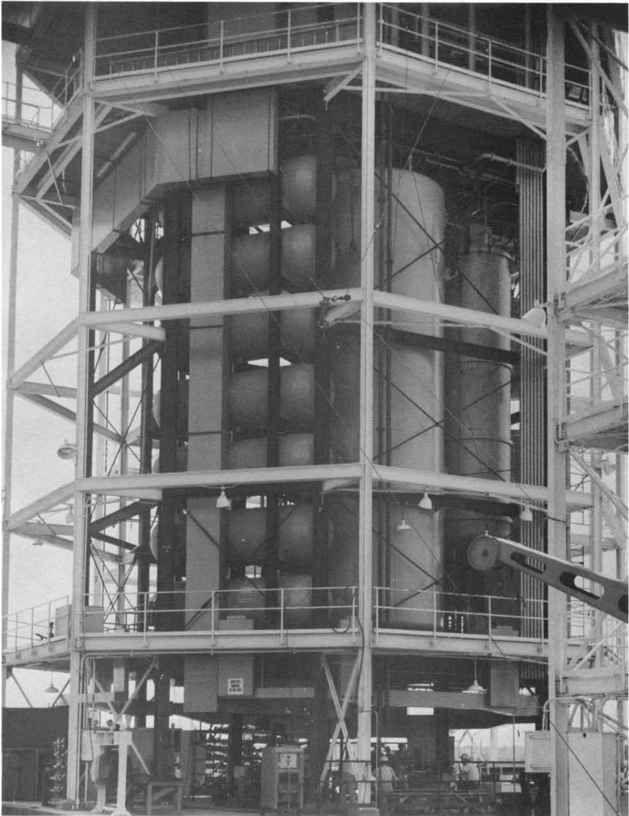
Tank farm from ground (Neg. No. 53923A dated 8-16-60).
