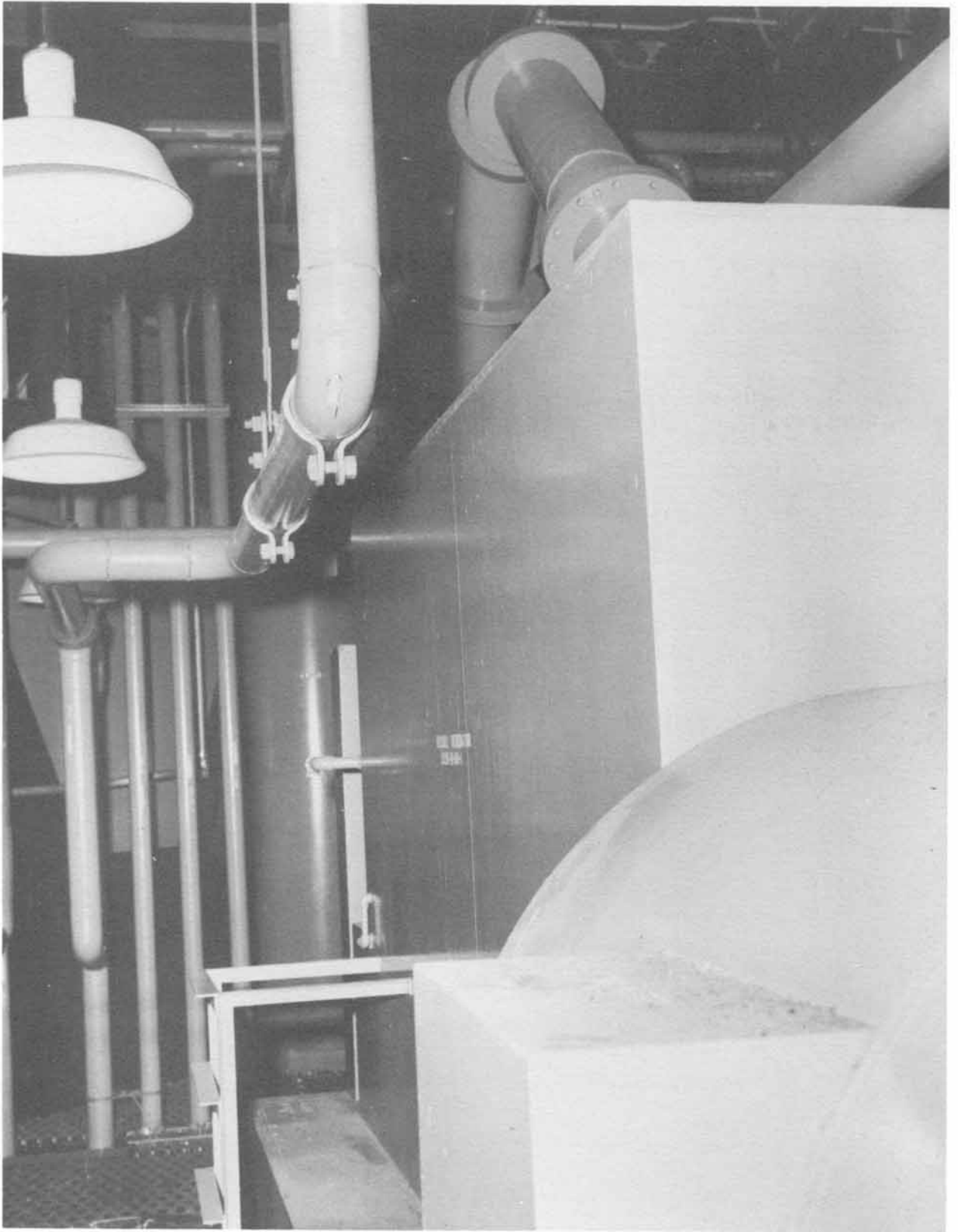
Piping on west side of diesel generator (Neg. No. 61633A dated 1-5-61).
