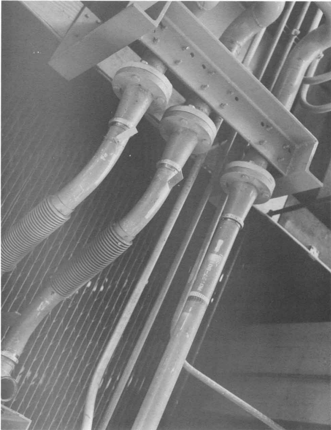
Power distribution unit facility interface Quad 3 below Level 8 (Neg. No. 67366A dated 4-14-61).
