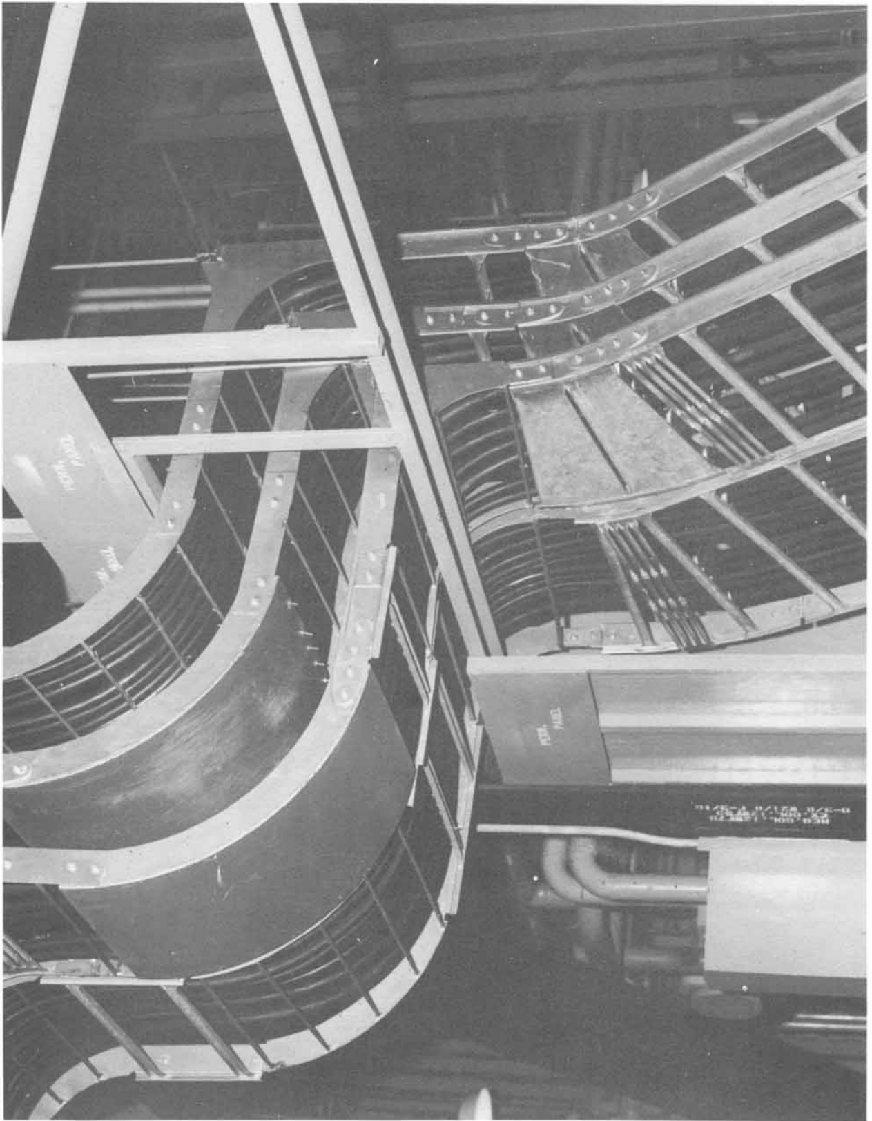
Umbilical loop shown extending through missile enclosure panels (Neg. No. 67564A dated 4-19-61).
