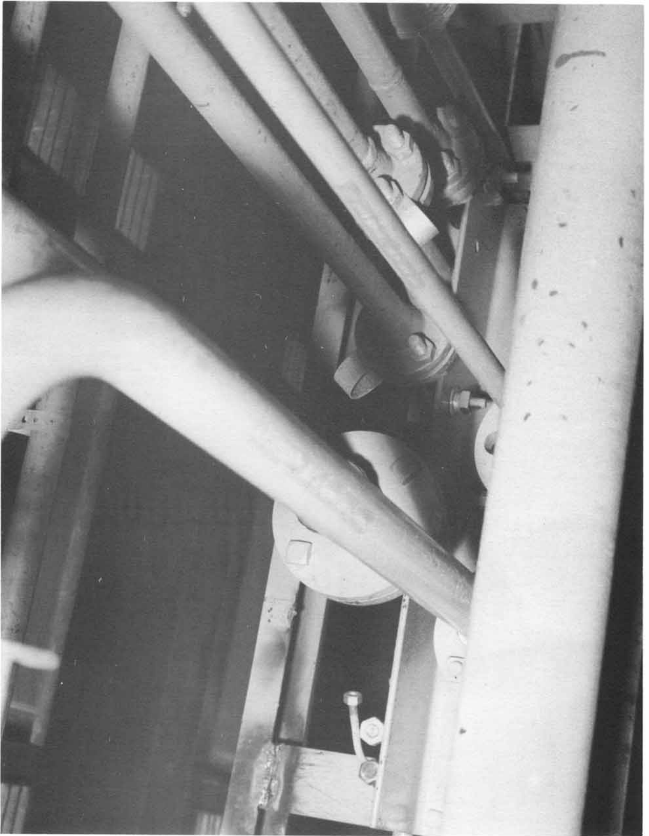
Pressurization control unit facility interface Quad 3 below Level 8 (Neg. No. 67367A dated 4-14-61).
