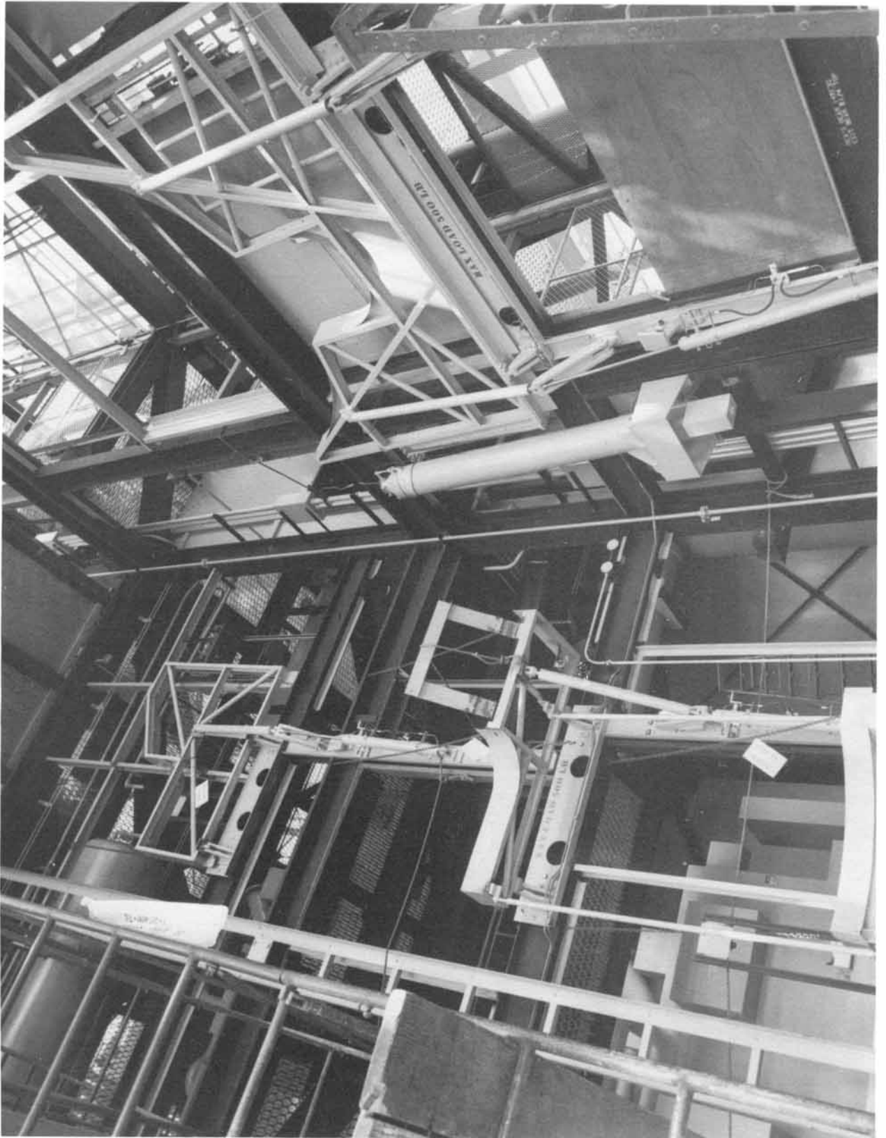
Collimator and work platforms (Neg. No. 53915A dated 8-16-60).
