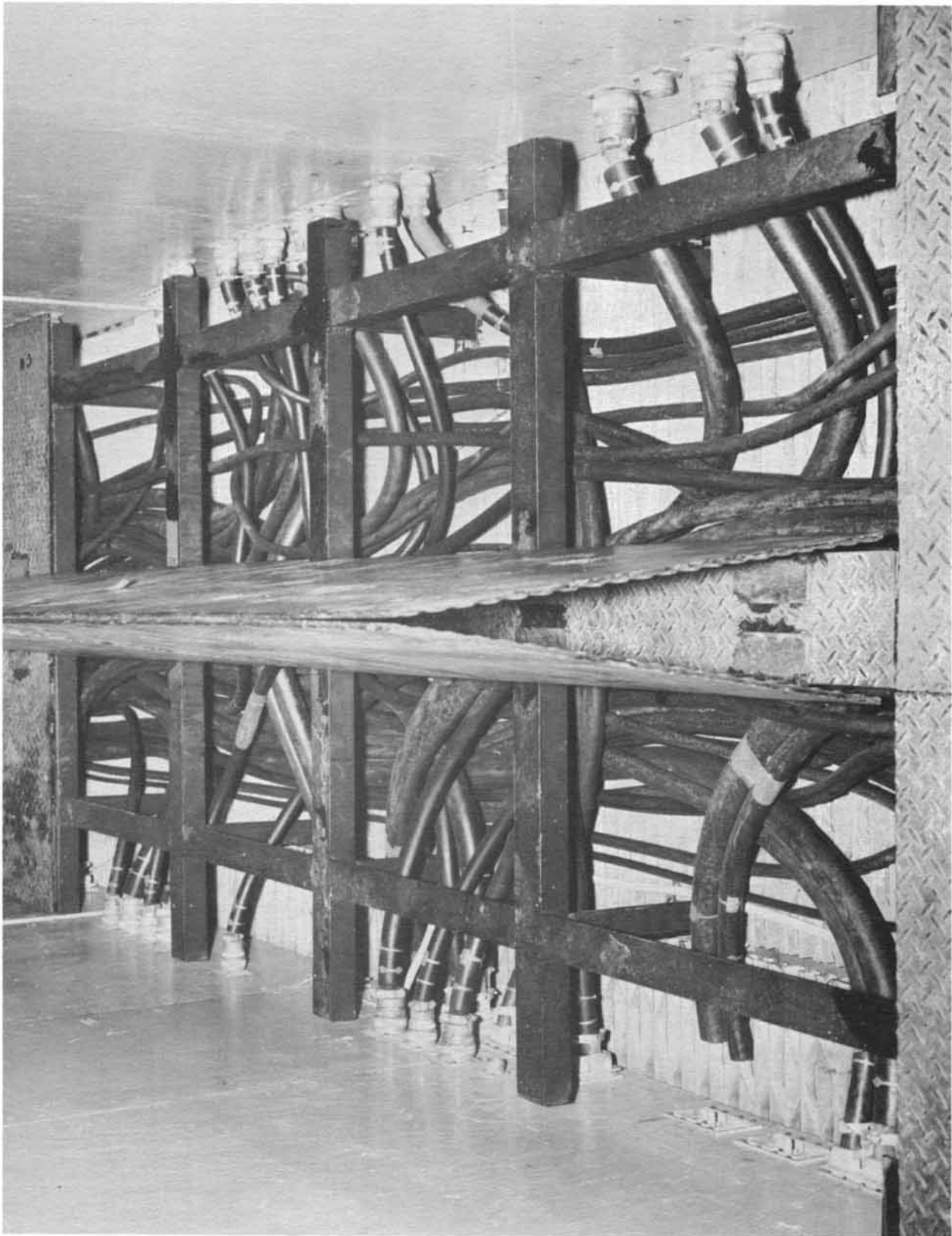
Cables under steel deck logic No. 2 to responder No. 2 (Neg. No. 55771A dated 9-27-60).
